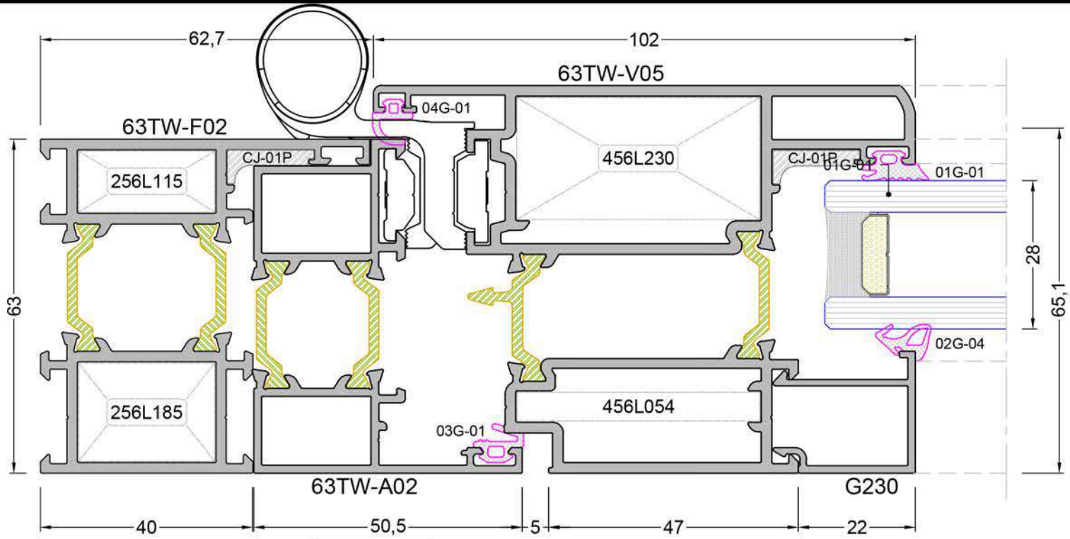
DETAY - 14 DETAIL - 14
