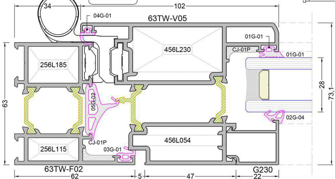
DETAY - 14c DETAIL - 14c
