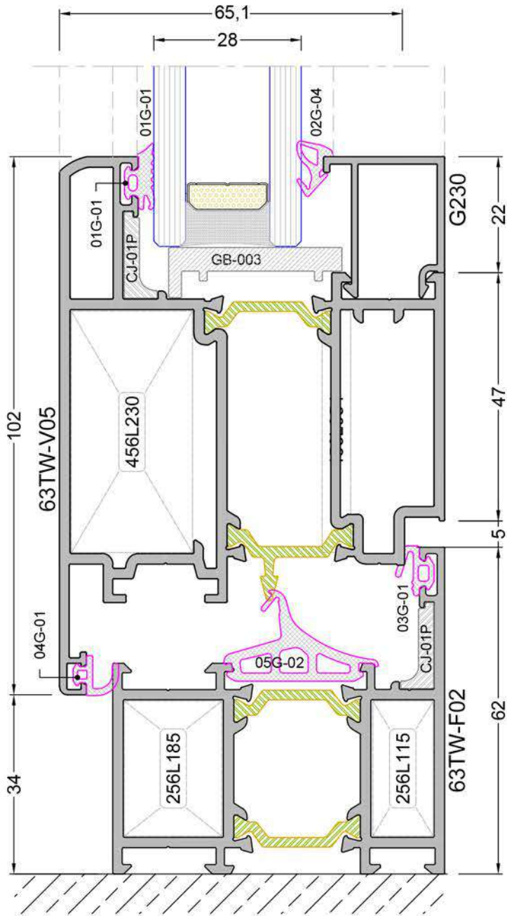
DETAY -16a DETAIL - 16a
