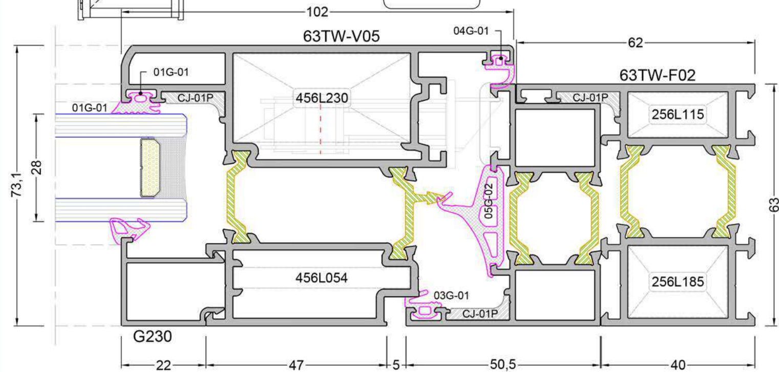
DETAY -17a DETAIL - 17a
