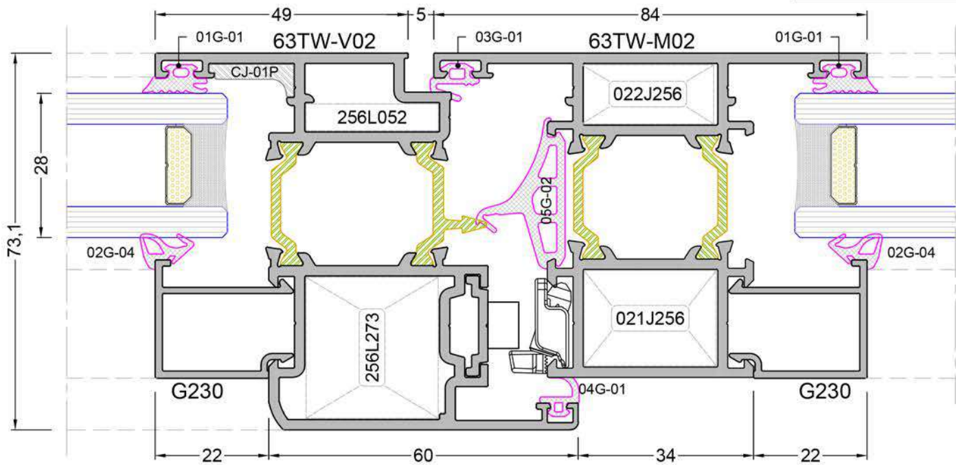
DETAY - 2 DETAIL - 2
