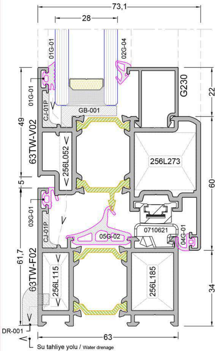
DETAY - 3 DETAIL - 3
