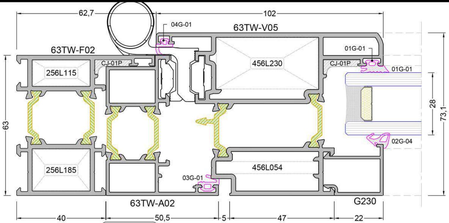
DETAY - 14b DETAIL - 14b
