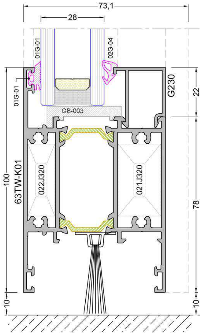
DETAY -16 DETAIL - 16
