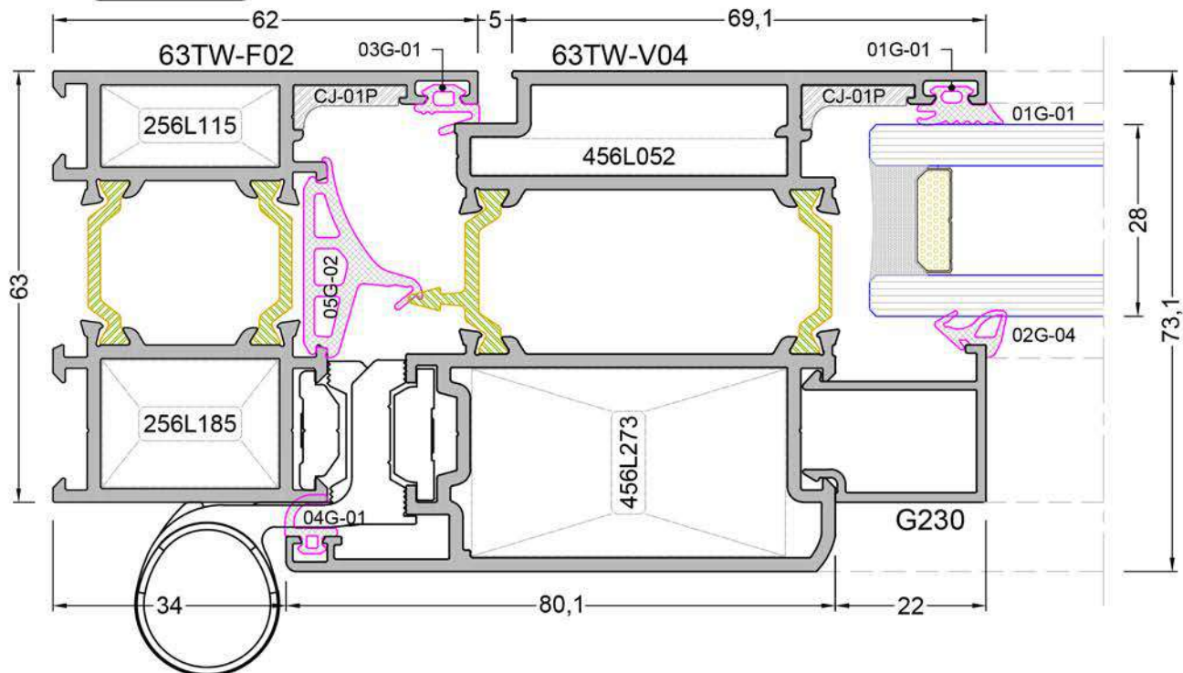
DETAY -10a DETAIL - 10a
