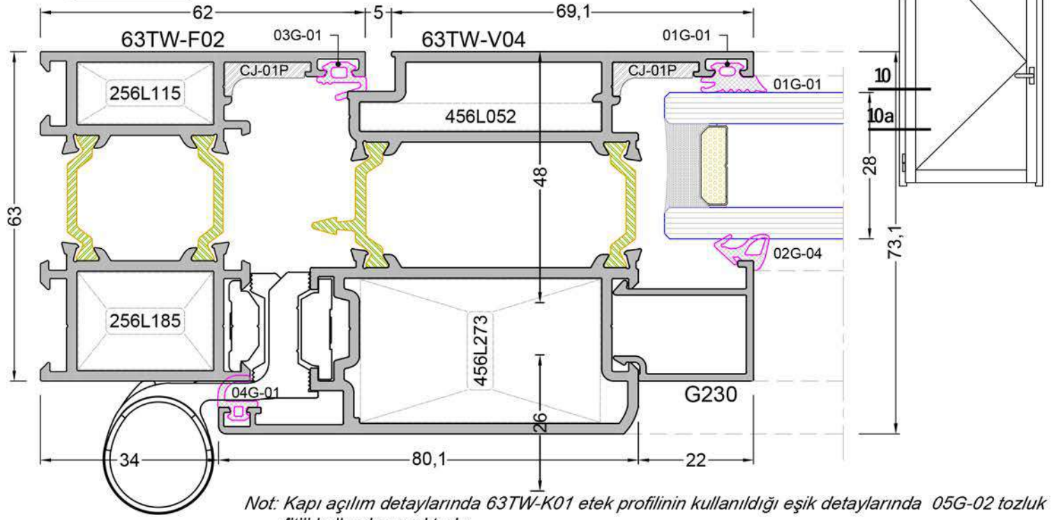
DETAY -10 DETAIL - 10
