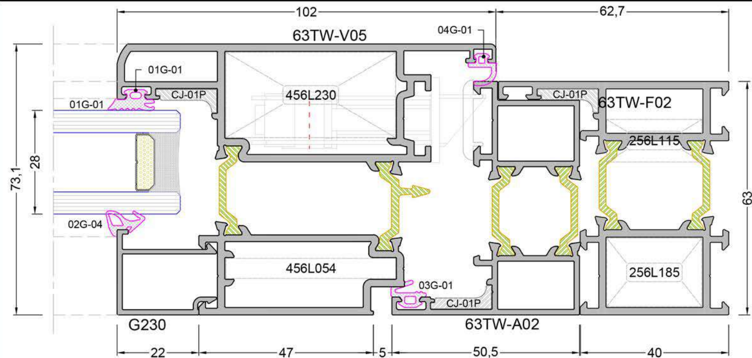
DETAY -17 DETAIL - 17
